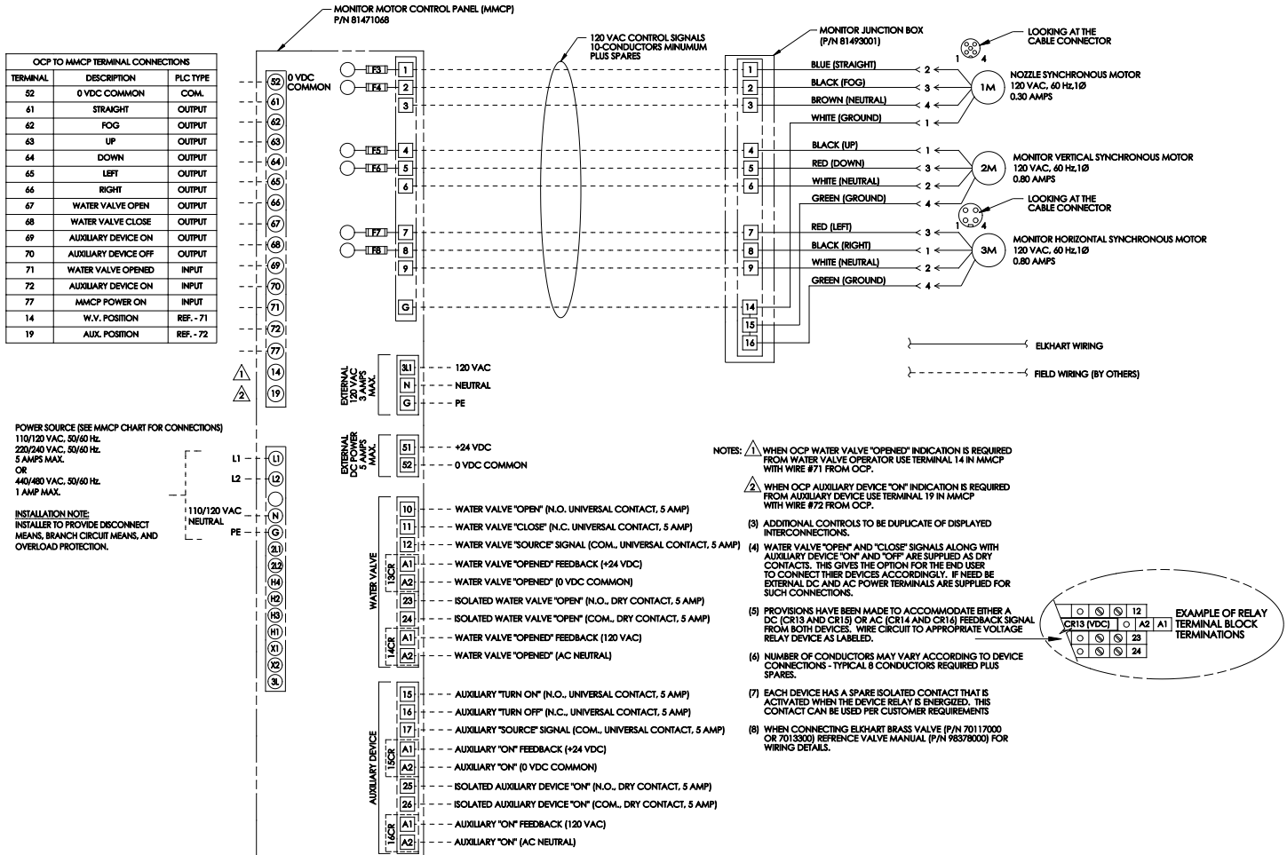
Figure 5: 81471068 MMCP/Monitor Motors - (Optional Valve and Auxiliary Device) Wiring Diagram
