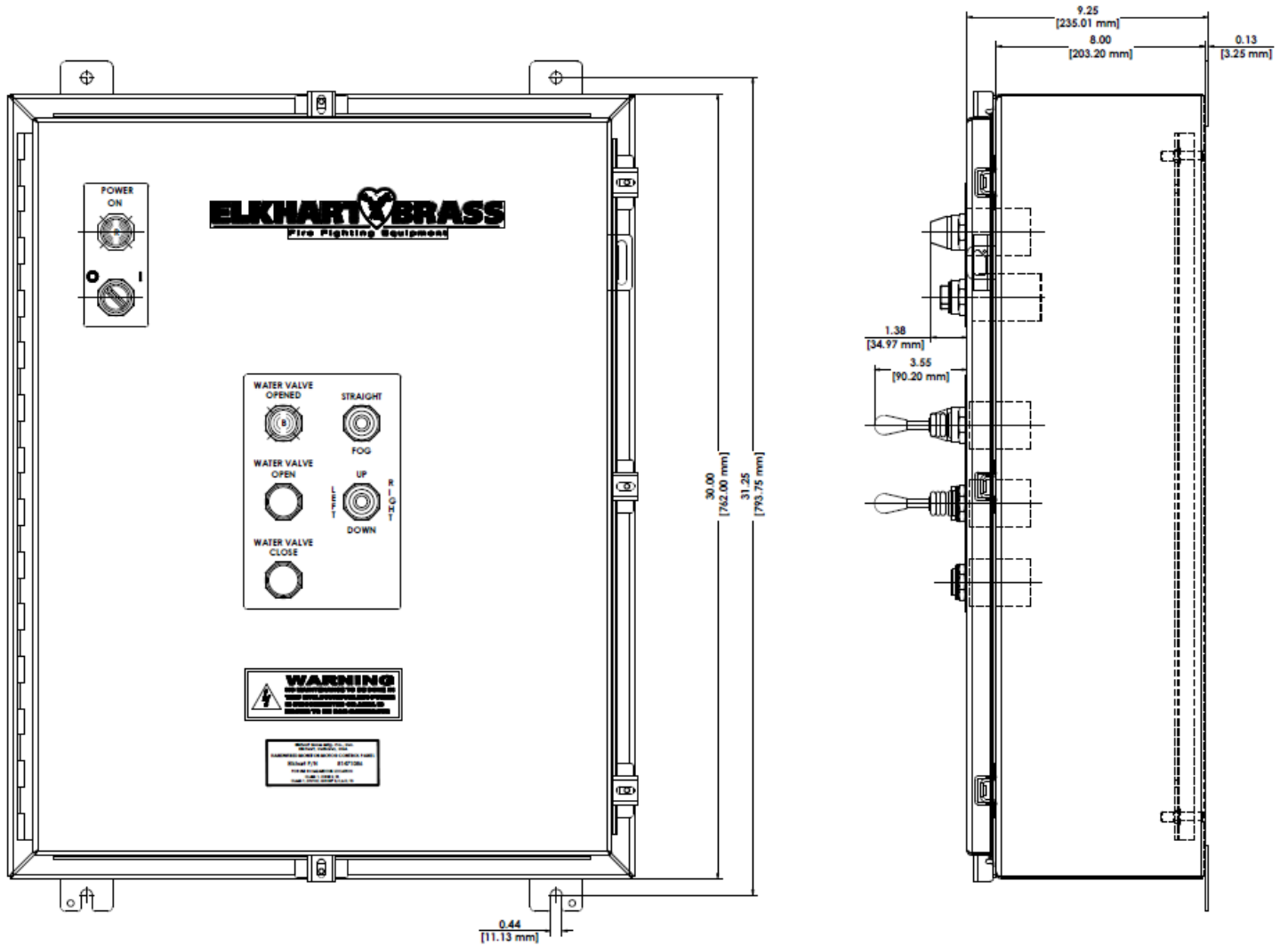
Figure 7: HMMCP Mounting Dimensions (814710856 shown)
