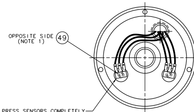
BOTTOM VIEW OF GEAR CASE COVER
