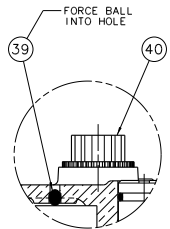
DETAIL A SCALE: 1 1/2 X SIZE
