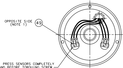
BOTTOM VIEW OF GEAR CASE COVER
