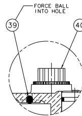
DETAIL A SCALE: 1 1/2 X SIZE
